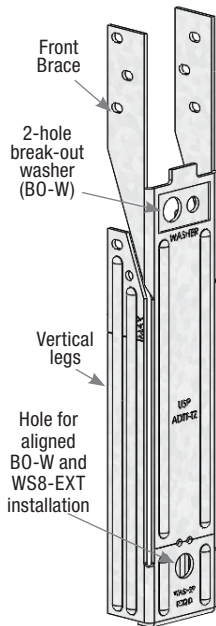
ADTT-TZ out of box
