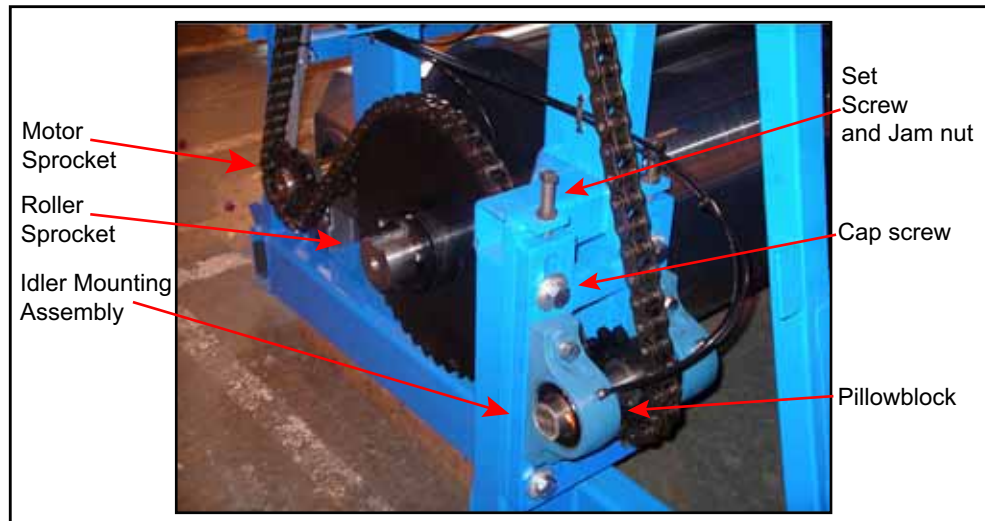
Figure 4: Finish Roller Drive System
