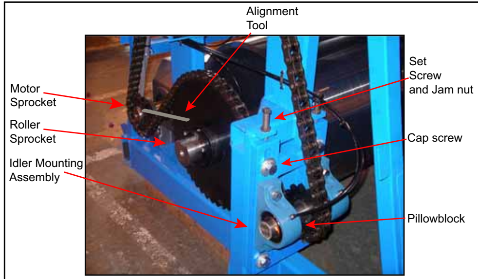
Figure 5: Drive System Alignment
