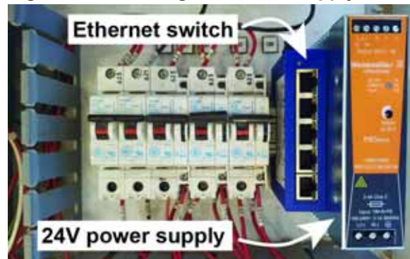
Figure 17: Mounting 24V Power Supply
