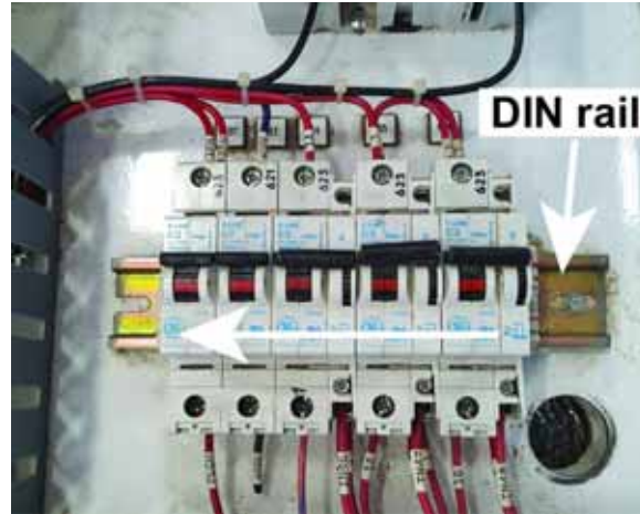
Figure 16: Shifting the Circuit Breakers
