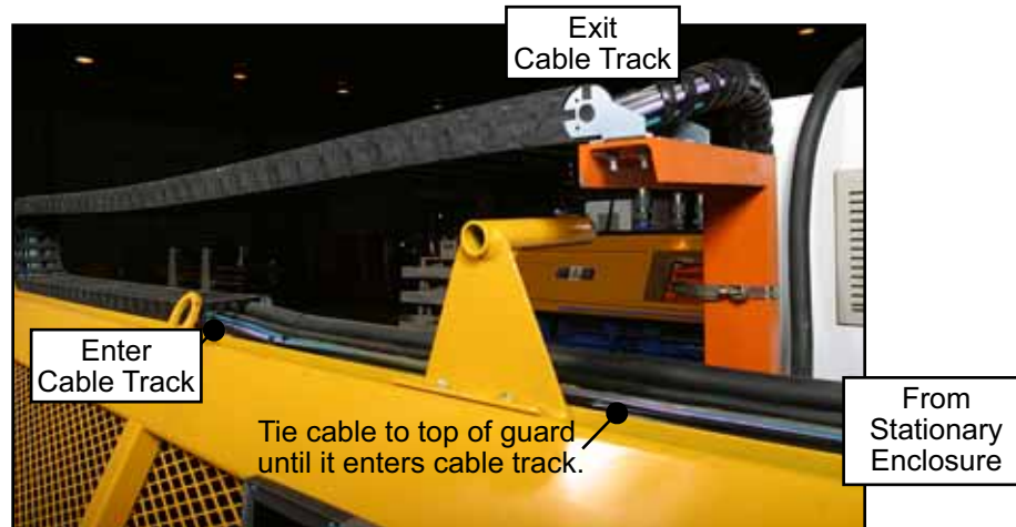
Figure 8: Cable Track
