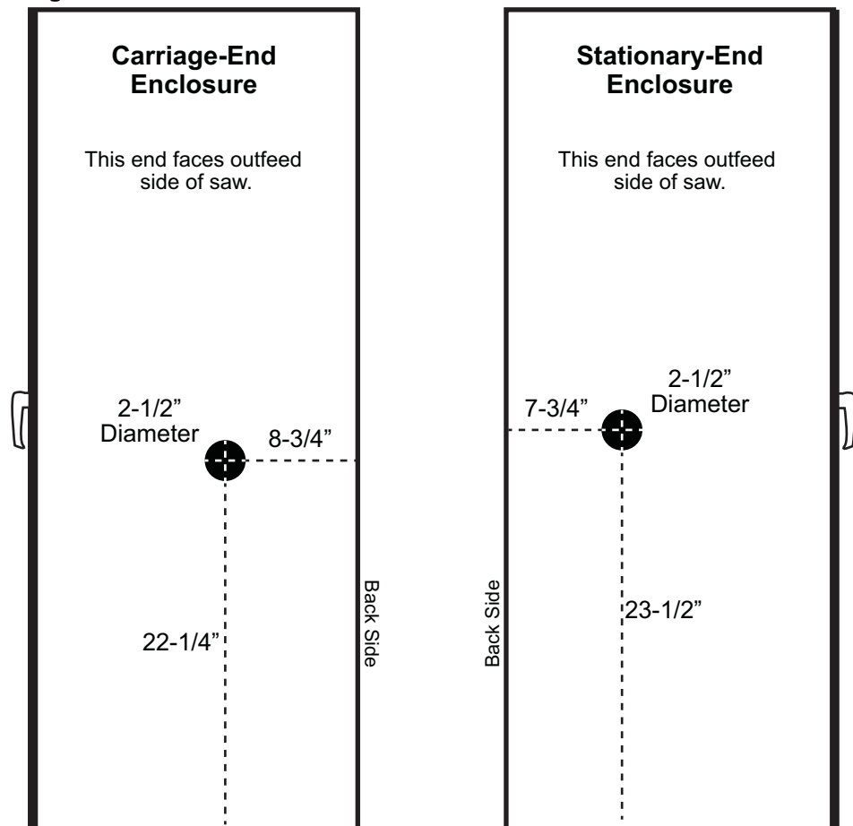
Figure 3: Hole Locations
