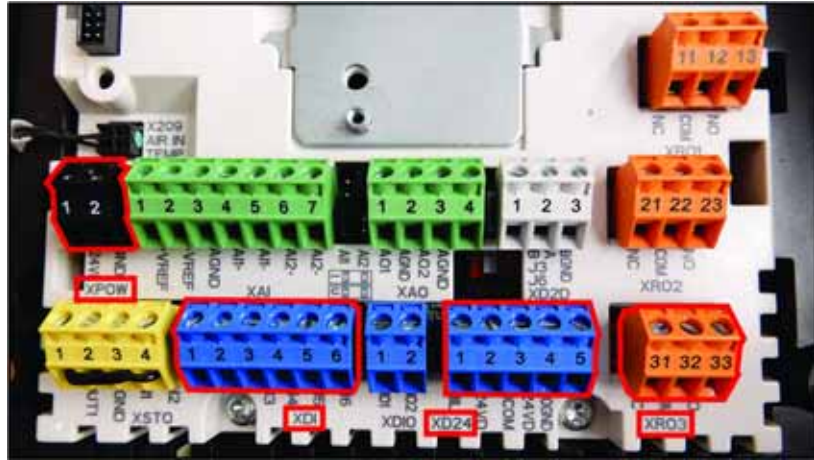
Figure 17: Terminal Blocks
