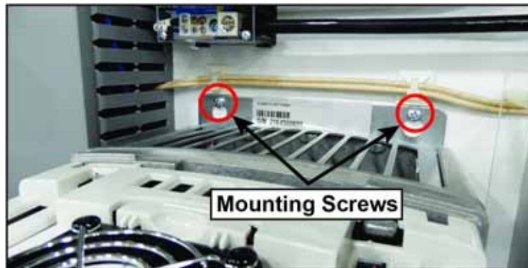
Figure 11: Top Mounting Screw Locations
