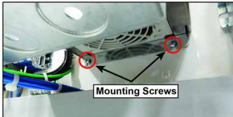
Figure 10: Bottom Mounting Screw Locations
