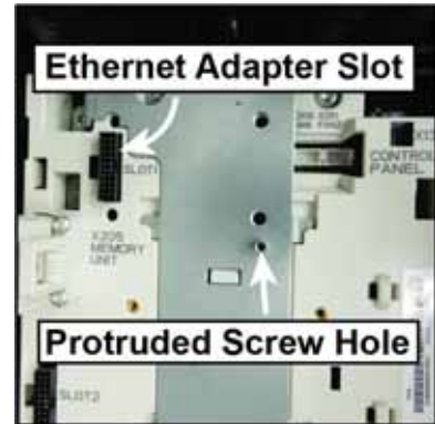
Figure 20: Ethernet Adapter Slot and Screw Locations
