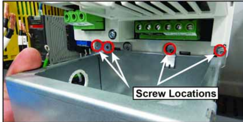
Figure 9: Wire Shield Screw Locations
