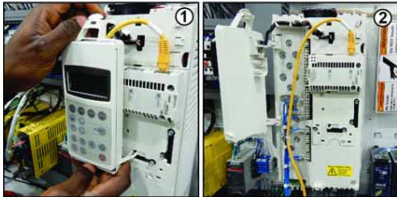
Figure 4: Exposing Wiring Behind the Keypad
