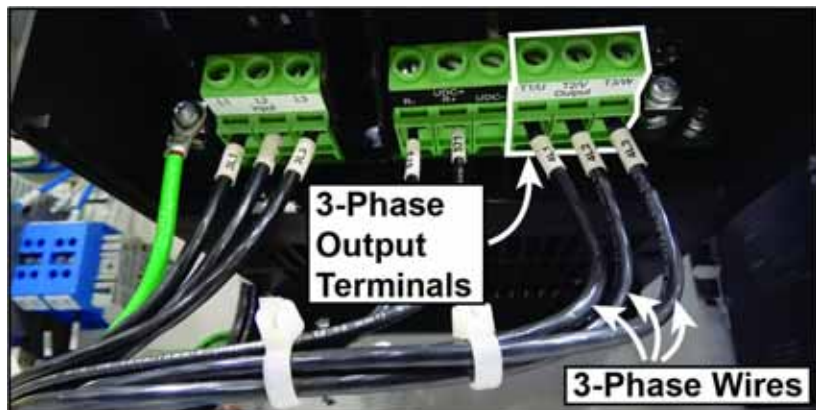
Figure 16: 3-Phase Output Wires.
