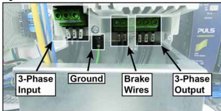
Figure 7: Wires on the Bottom of the VFD
