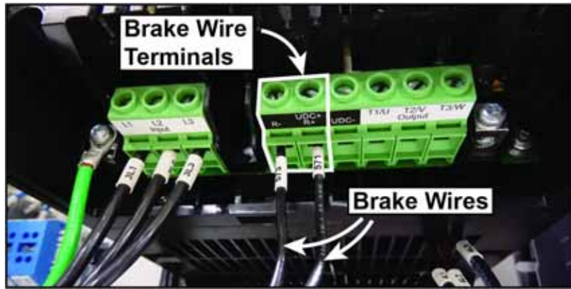
Figure 15: Brake Wires
